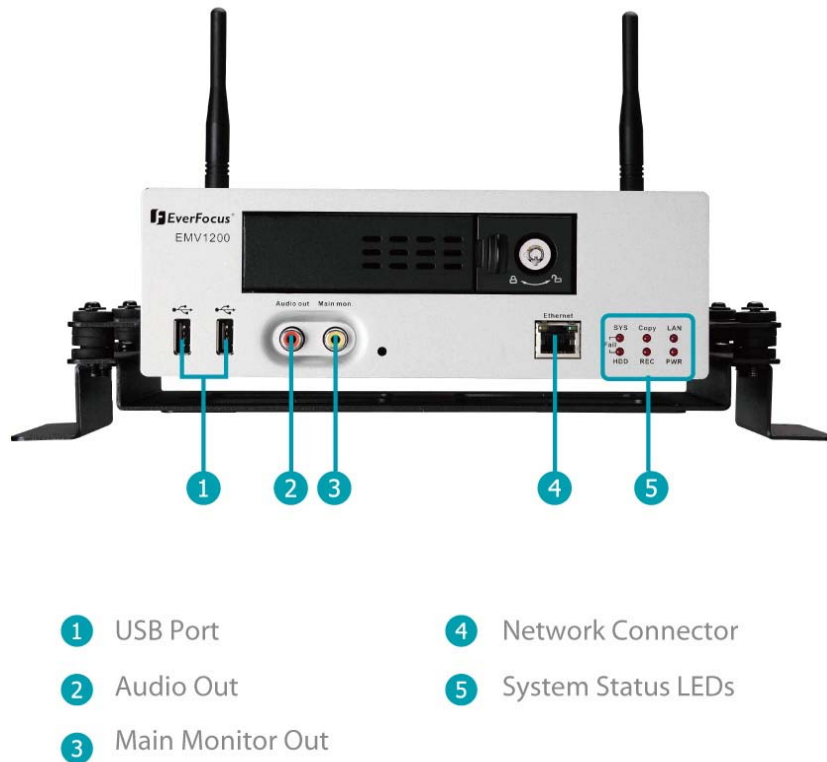
Figure 1-1 Front Panel
